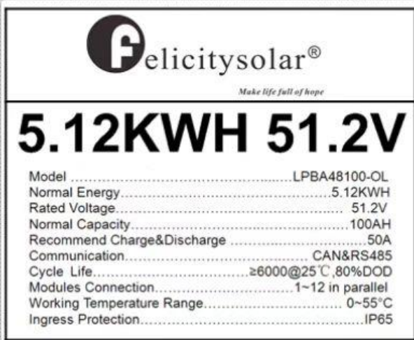
电池铭牌(含 Wh) Battery nameplate (With Wh)
