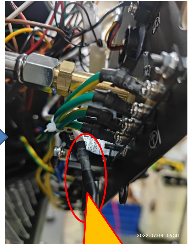
Wrap the removed white wire terminal with insulating tape, and then restore the unit to complete the operation of canceling the neutral grounding.
